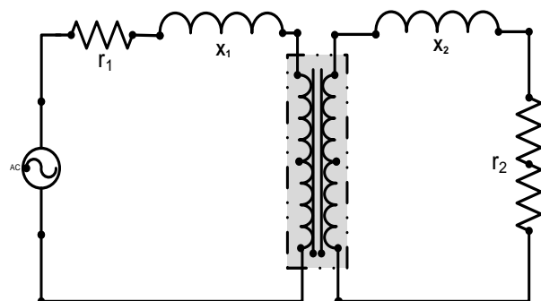
Fig.1 Basic circuit of induction motor
