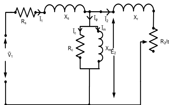
Fig. 2 Equivalent circuit of induction motor
