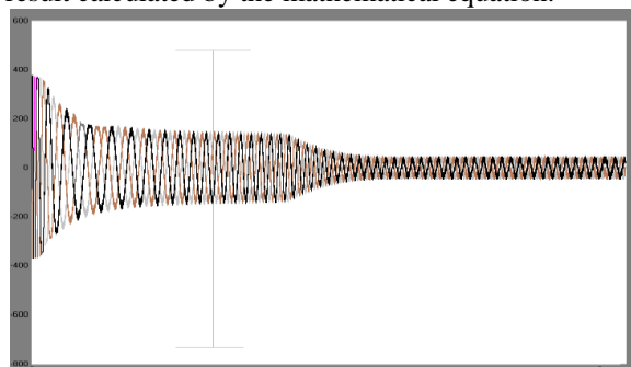
Fig.5 Current Vs. Time Curve for SCIM
