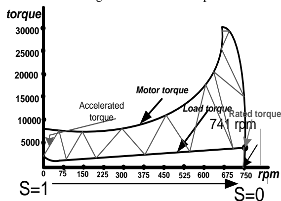
Fig.3 torque vs. speed curve of induction motor.
