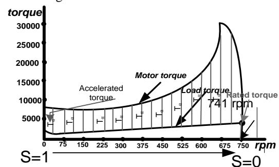
Fig. 4 torque vs. speed curve of induction motor when is complex.
